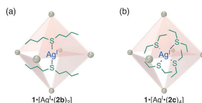
Figure 3. Silver–dialkyl sulfide complexes within cage 1 : a) 1\cdot[\text{Ag}^+(\text{2b})_2] , b) 1\cdot[\text{Ag}^+(\text{2c})_4] .
